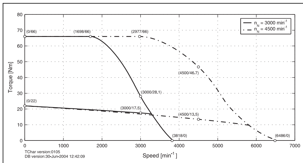
Figure 23: Speed - torque characteristic curve for 8MSA5E.dd-eeff-1
