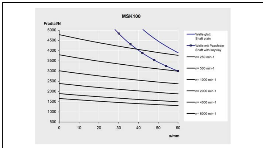
Fig. 4-103: permissible radial force of MSK100 - Motors (shaft and bearing load)
