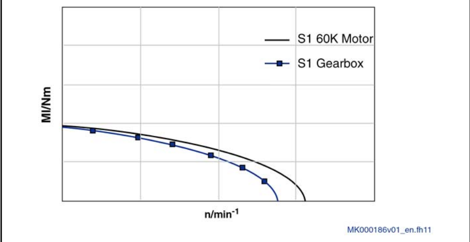
Fig. 9-17: S1 characteristic curve of gearboxes
