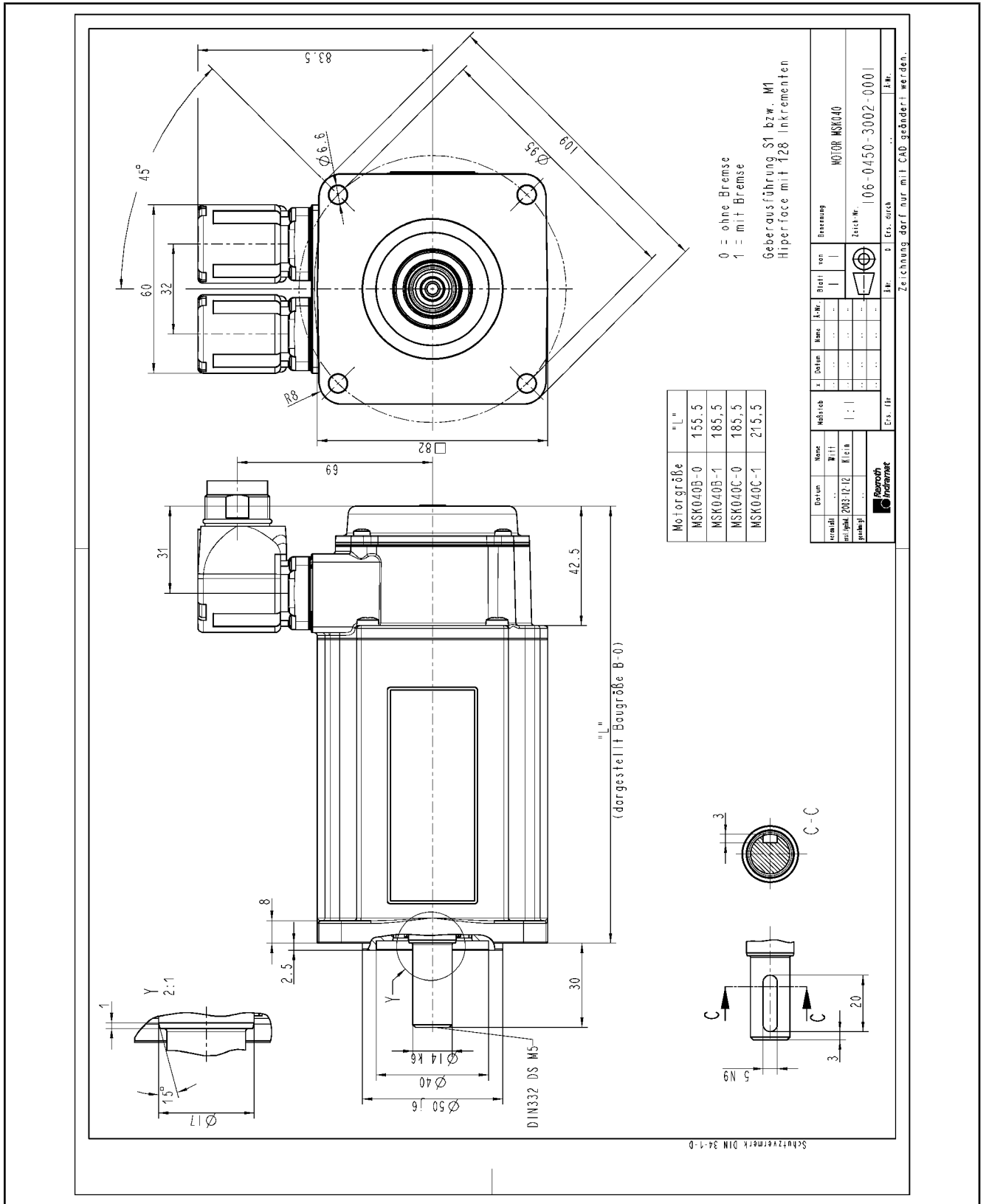
Fig. 5-4: MSK040 specification
