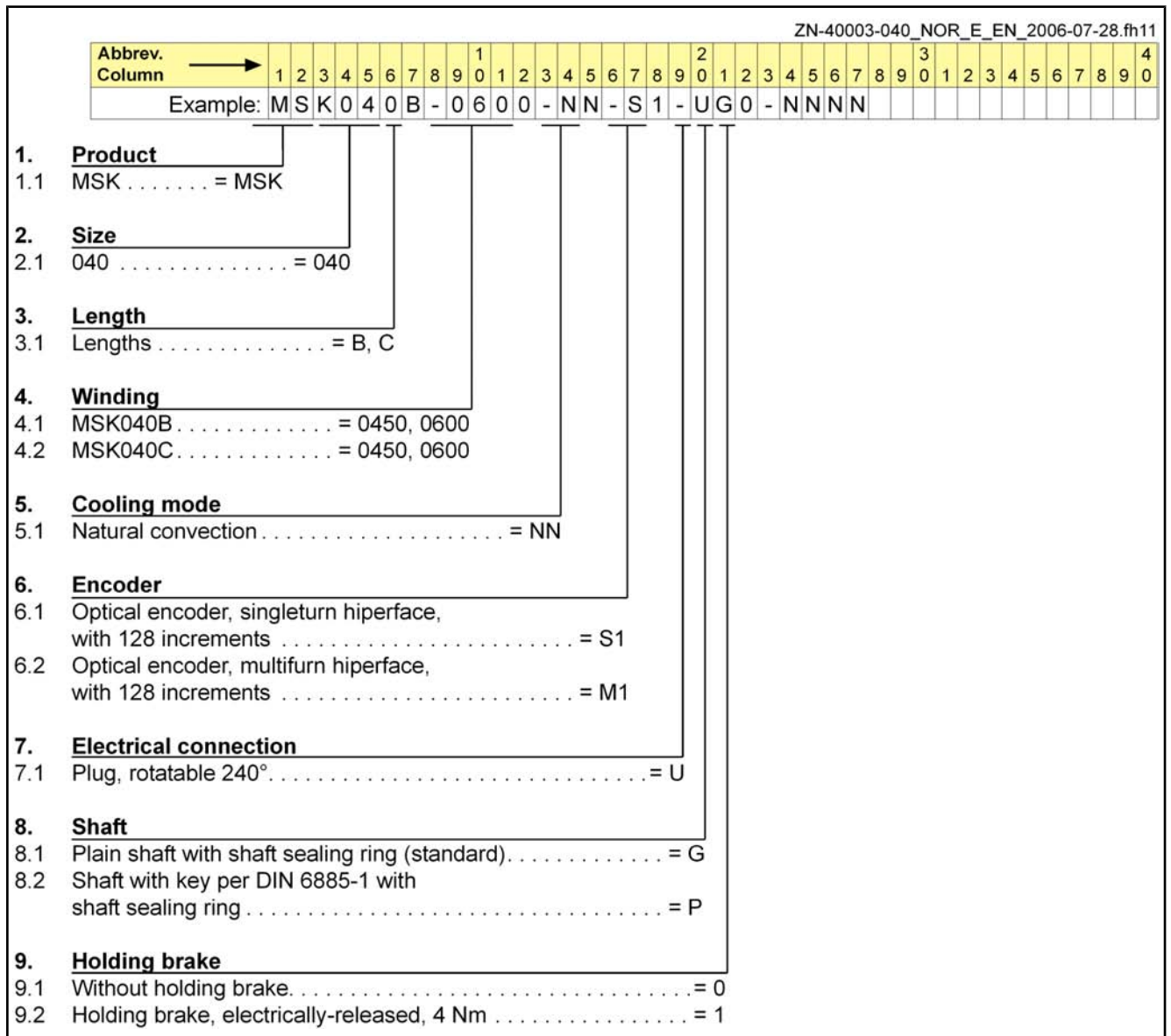
Fig. 6-8: Type Codes MSK040 (page 1)
