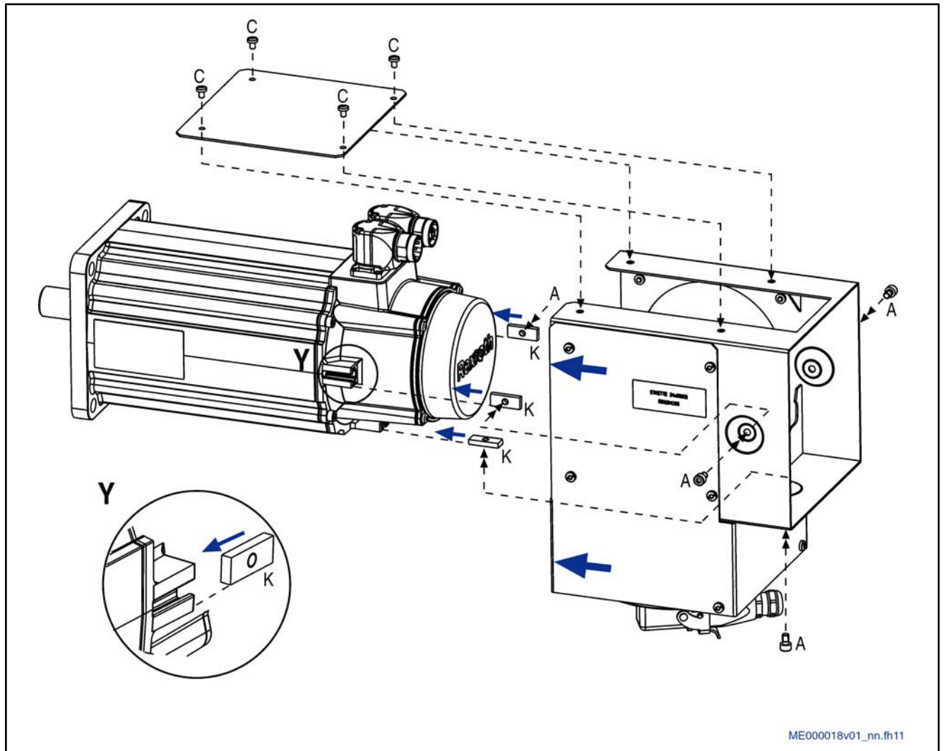
Fig.7-30: Assembly of fan units LEM-RB-116N-xx-NNNN, LEM-RB-140N-xx-NNNN
