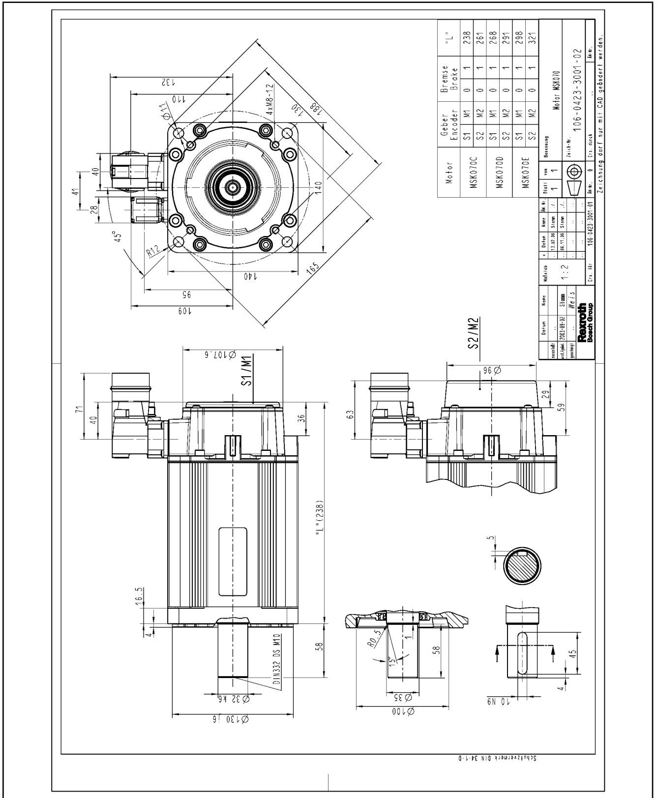
Fig.5-8: MSK070 specification
