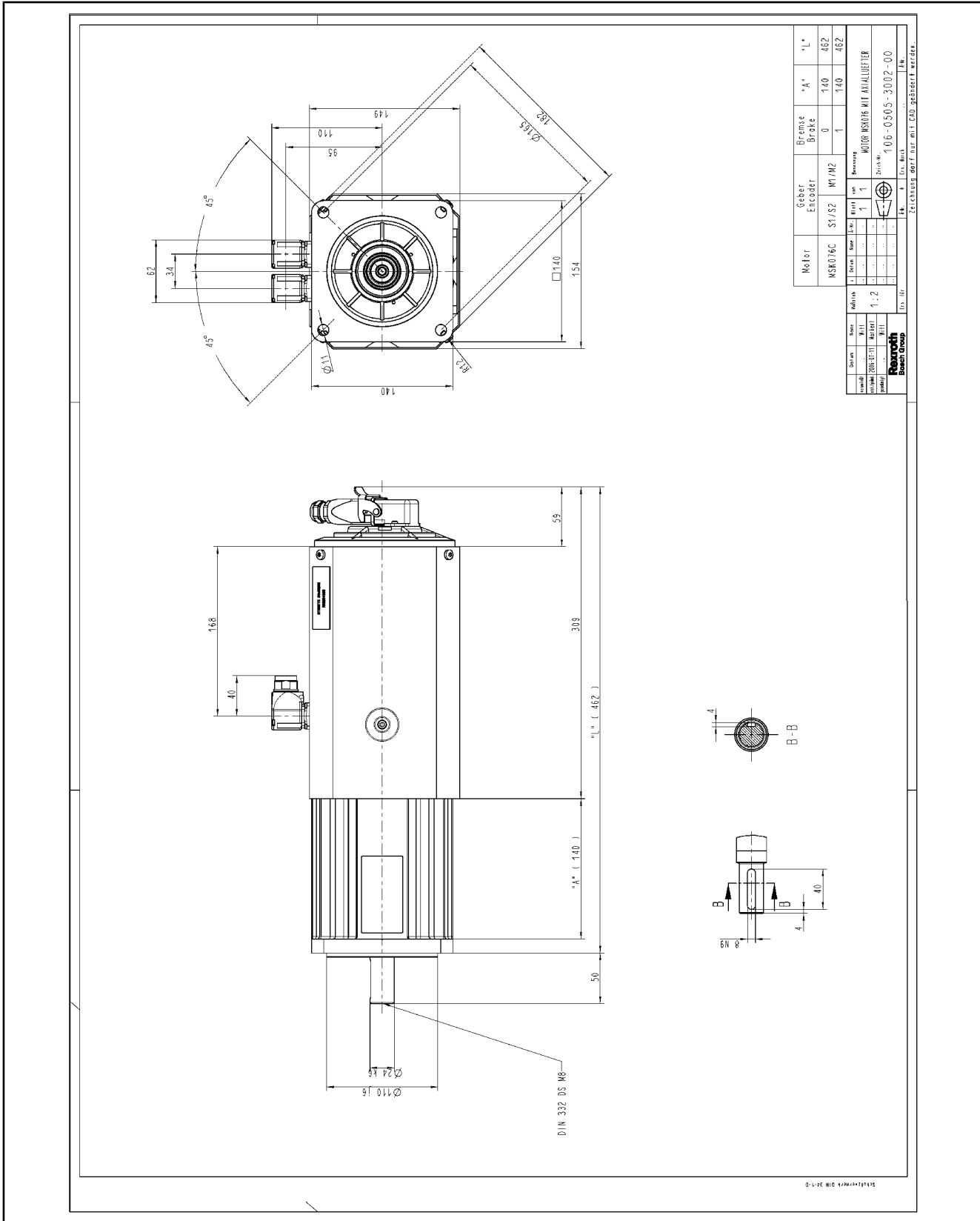
Fig.7-16: Dimension sheet MSK076 with axial fan unit
