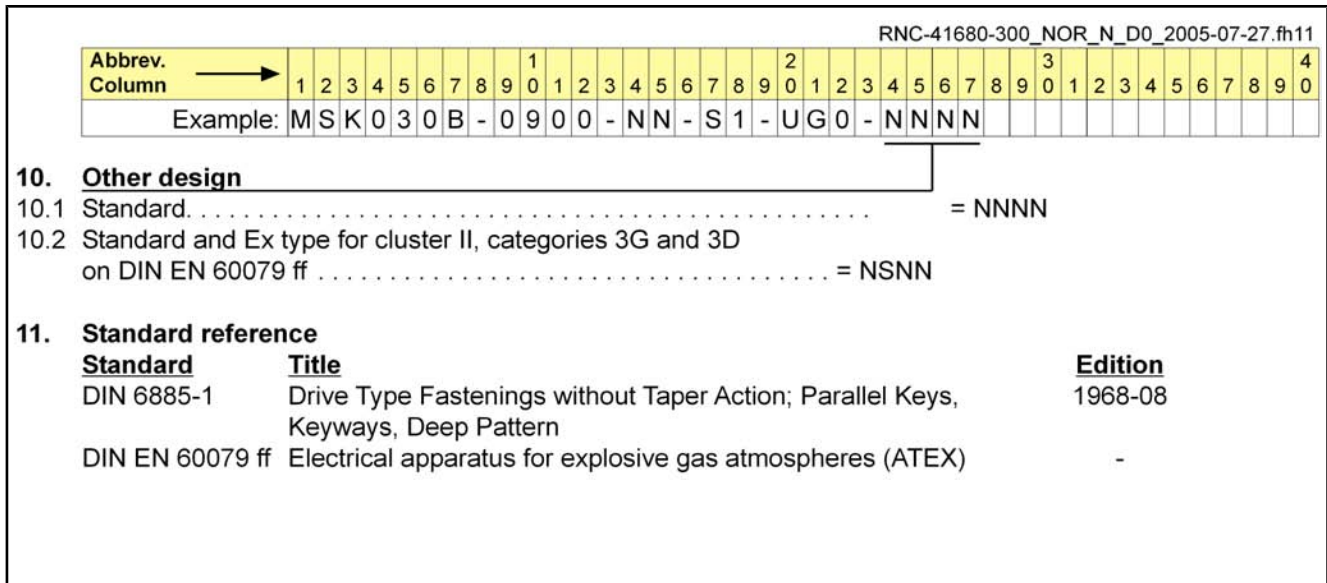
Fig.6-7: Type Codes MSK030 (page 2)
