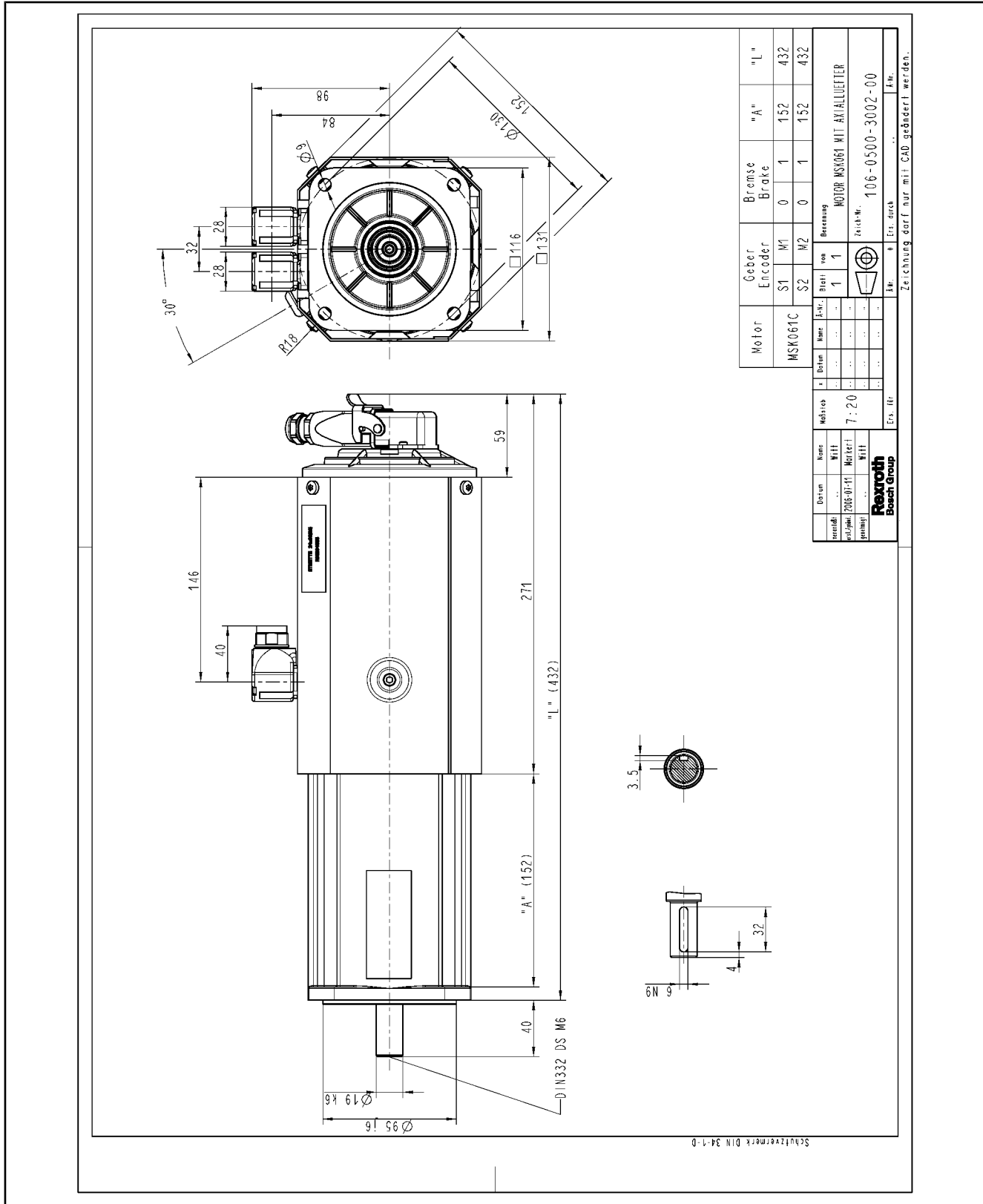
Fig.7-10: Dimension sheet MSK061 with axial fan unit
