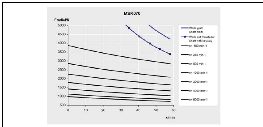
Fig.4-58: permissible radial force of MSK070 - Motors (shaft and bearing load)
