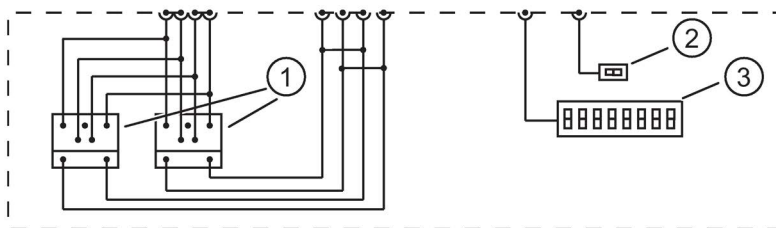
Figure 12-1 Block diagram of CM IM DP ECOFAST Cu for interface modules
