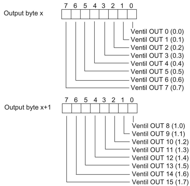
Figure A-30 Address range 16 DO DC24V
