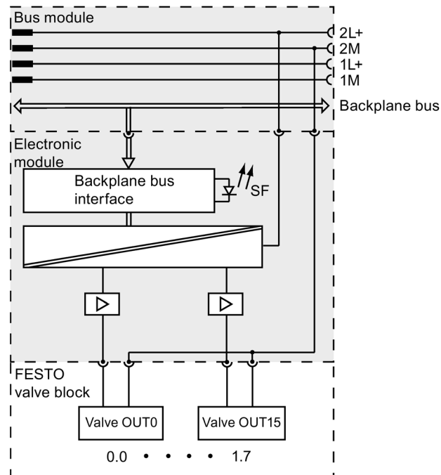
Figure 17-1 Block diagram 16 DO DC 24V CPV10
