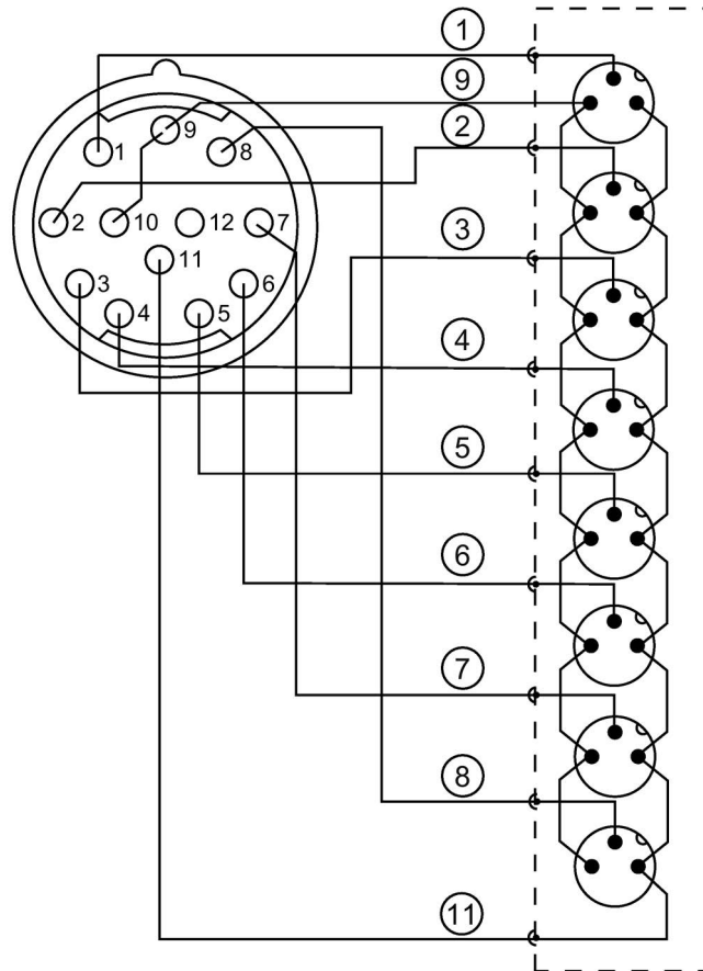
Figure A-37 Actuator/sensor distributor to digital inputs with connection module CM IO 1 x M23
