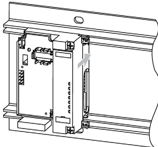
Figure 4-6 Mounting the interface module for PROFIBUS DP (example)
