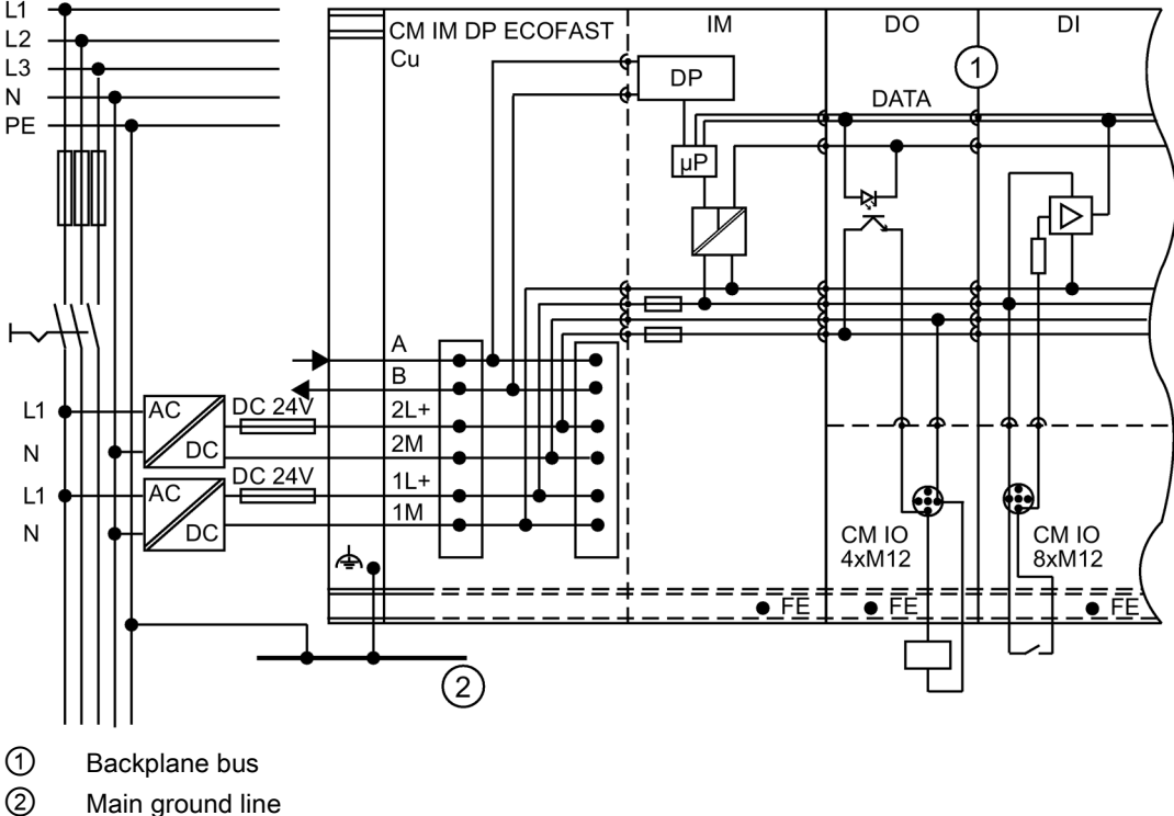
Figure 5-2 ET 200pro configuration with CM IM DP ECOFAST Cu connection module
