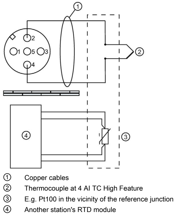
Figure A-44 Connection example based on "Dynamic ref. temp." as the reference junction
