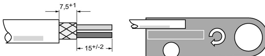
Figure 5-7 Stripping dimensions for the PROFIBUS DP cable
