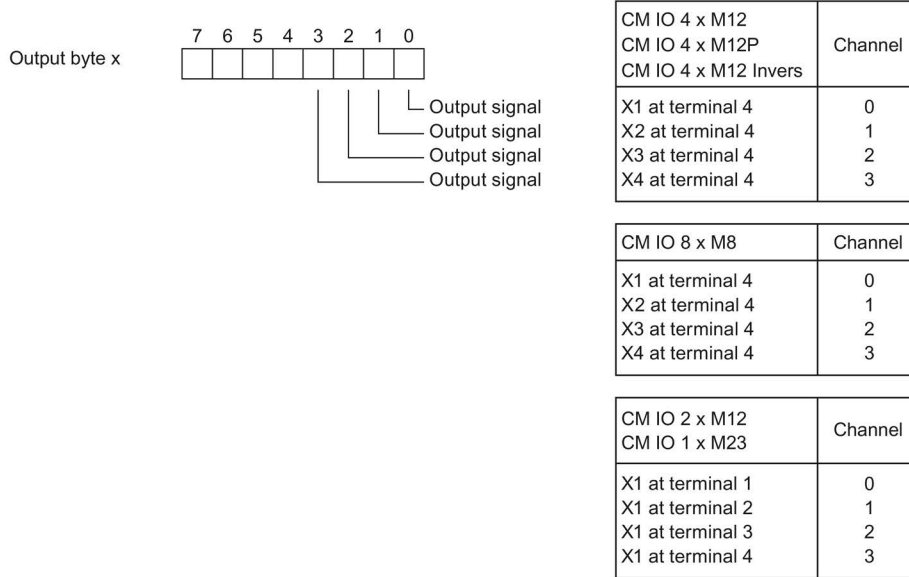
Figure A-23 Address space 4 DO DC 24V/0.2A
