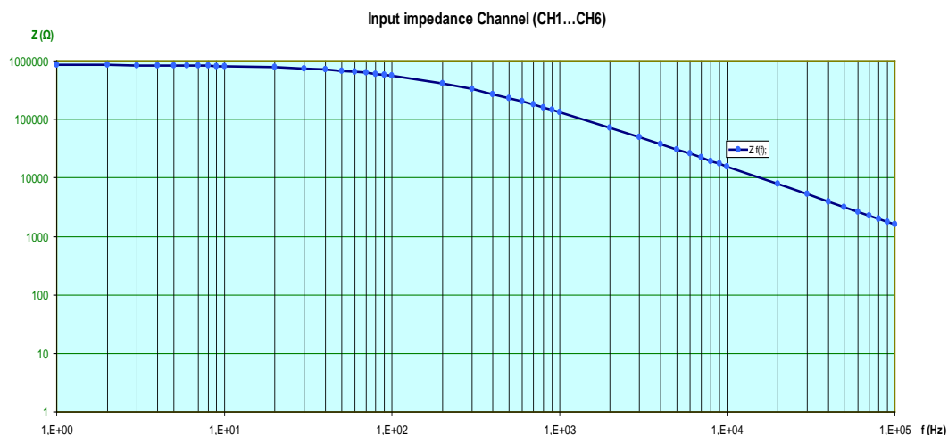
Bild 16 Input impedance channels (CH1...CH6)
