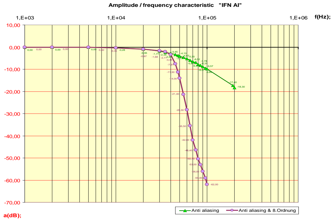
Bild 15 filter characteristic (CH1...CH6)
