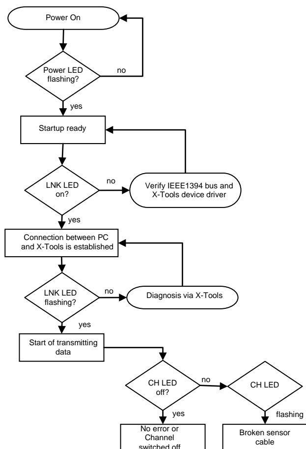
Picture 12 Start-up IFN AI
