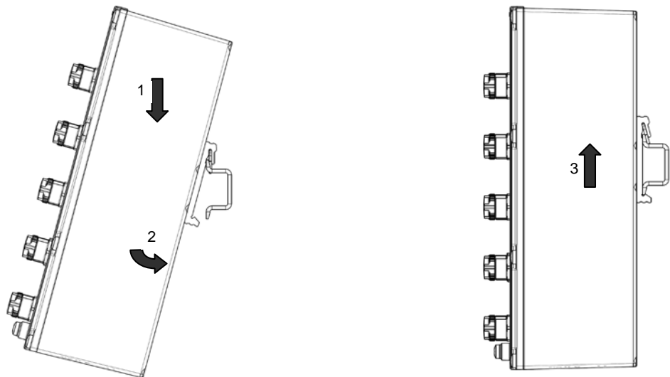
Picture 4 Installation of the device IFN AI on a DIN rail.
