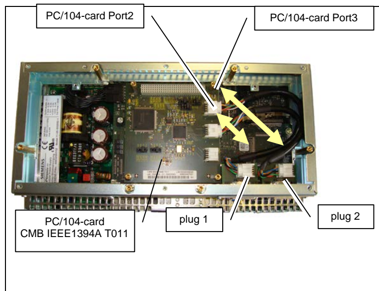
Picture 14 MICROBOX PC with CMB IEEE1394A
