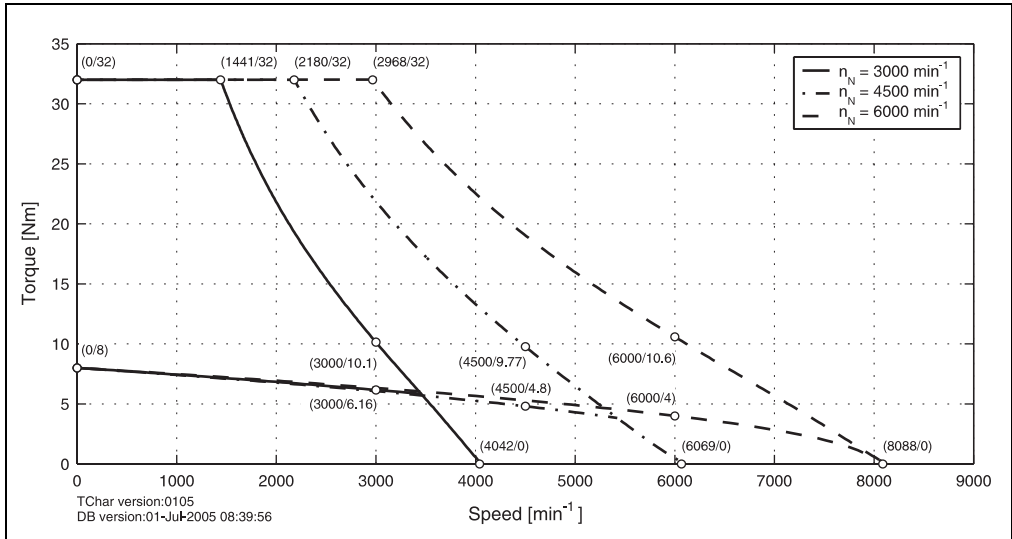
Figure 25: Speed - torque characteristic curve for 8LSA45.eennffgg-0
