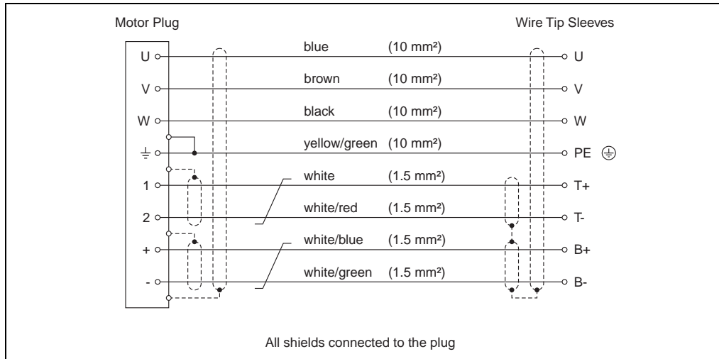
Figure 68: Cable schematic for motor cables 8CMxxx.12-5
