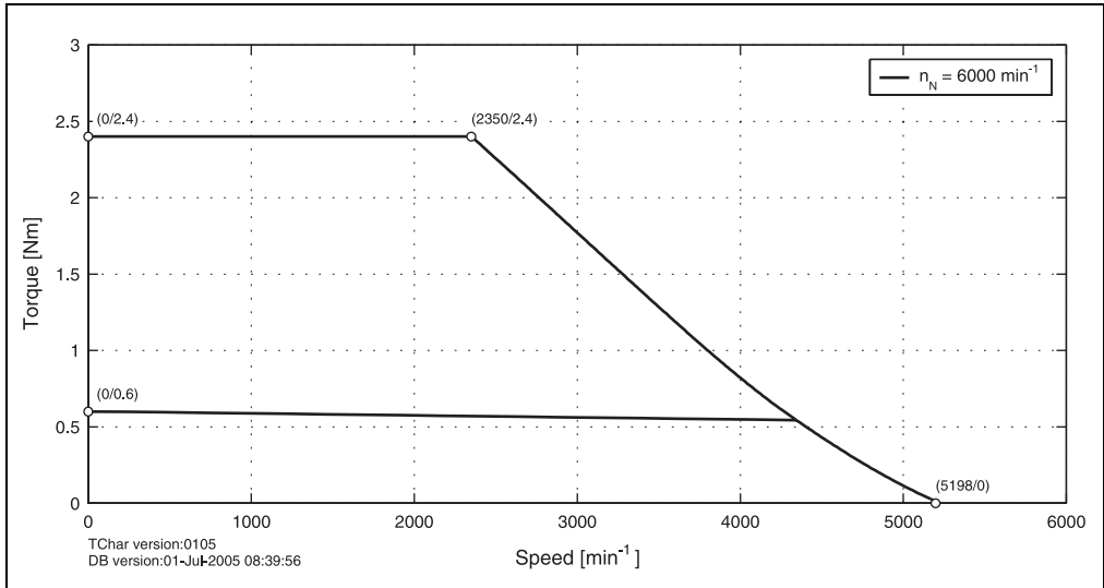
Figure 13: Speed - torque characteristic curve for 8LSA25.eennffgg-0
