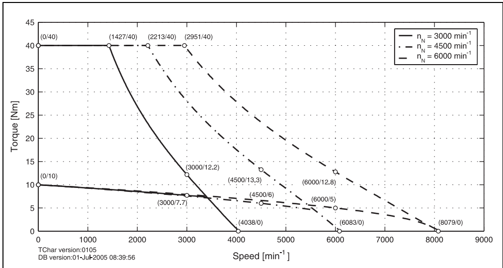
Figure 26: Speed - torque characteristic curve for 8LSA46.eennffgg-0
