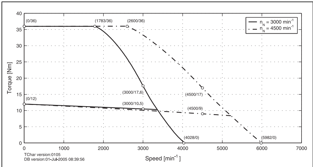
Figure 33: Speed - torque characteristic curve for 8LSA55.eennnffgg-0
