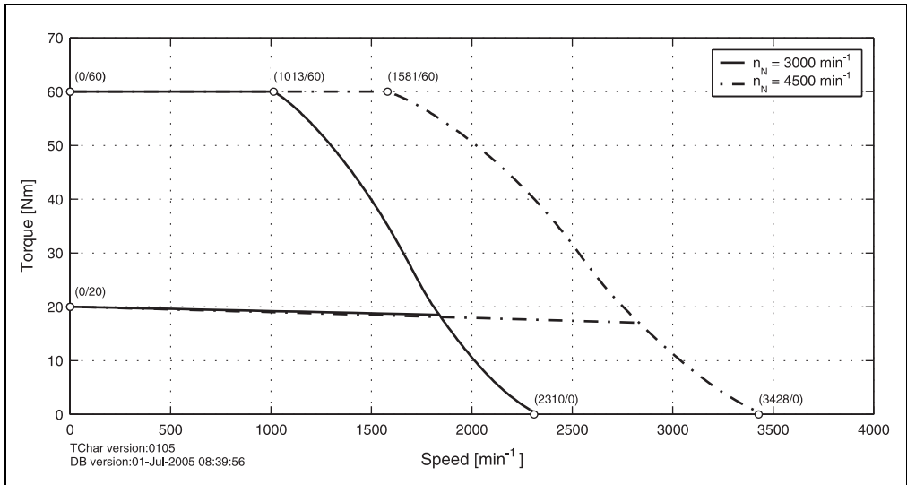
Figure 40: Speed - torque characteristic curve for 8LSA57.eennffgg-0
