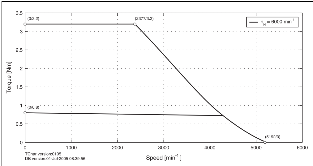
Figure 14: Speed - torque characteristic curve for 8LSA26.eennffgg-0
