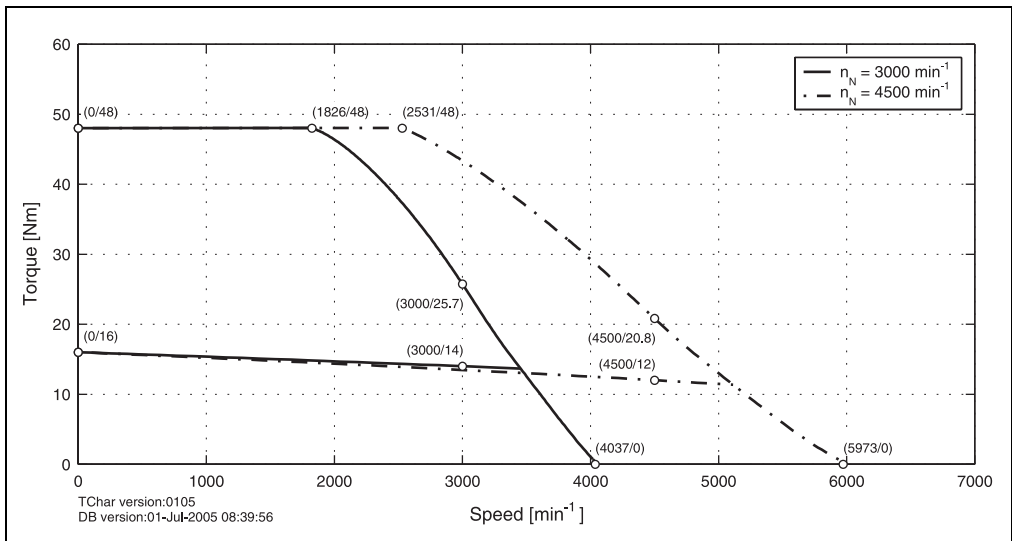
Figure 34: Speed - torque characteristic curve for 8LSA56.eennnffgg-0
