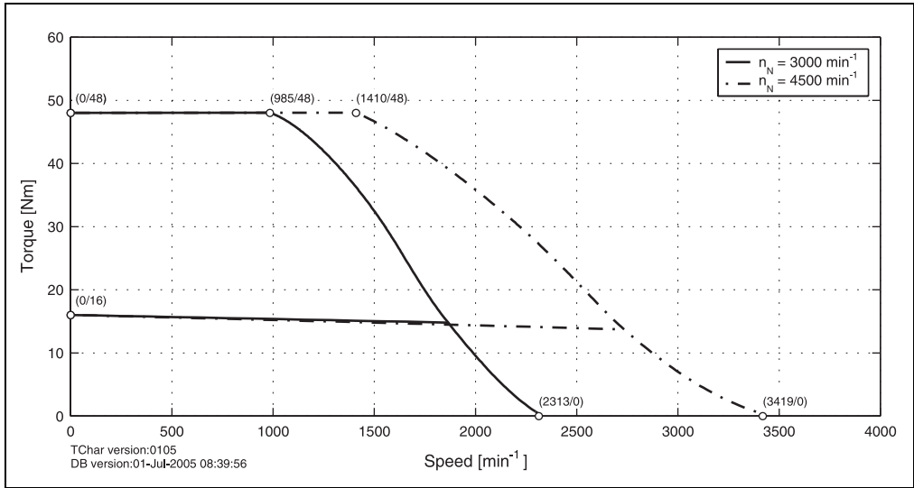
Figure 39: Speed - torque characteristic curve for 8LSA56.eennffgg-0
