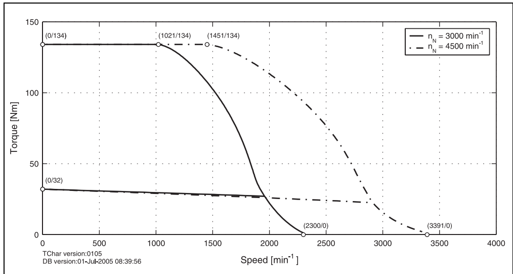
Figure 53: Speed - torque characteristic curve for 8LSA74.eennnffgg-0
