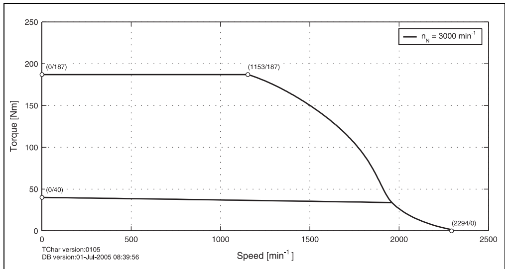
Figure 54: Speed - torque characteristic curve for 8LSA75.eennnffgg-0
