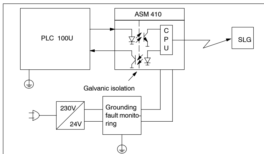
Figure 3-25 SIMATIC PLC 100U with ASM 410
