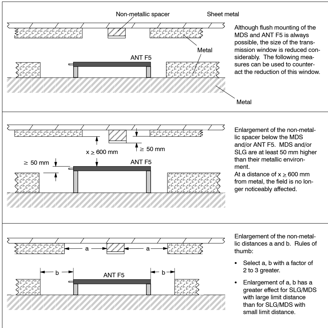
Figure 3-16 Flush installation
