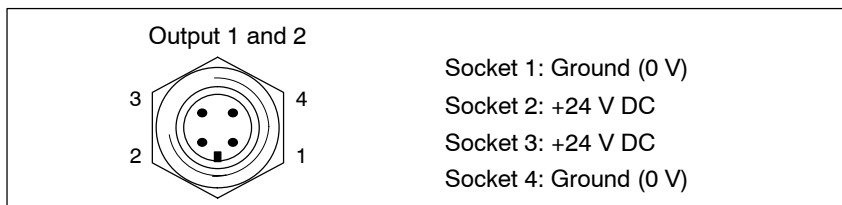
Figure 7-2 Plug connector allocation of 24 V output
