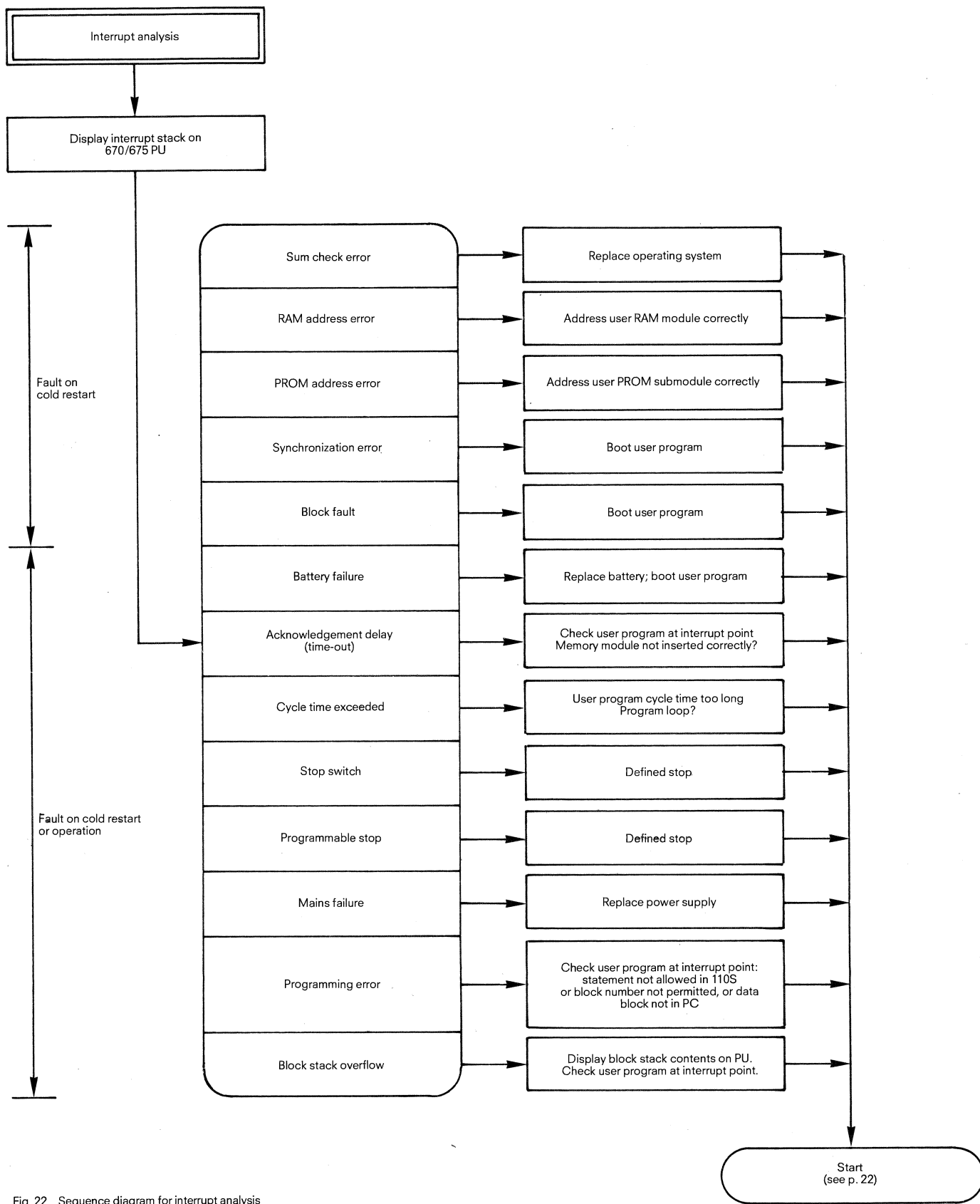
Fig. 22 Sequence diagram for interrupt analysis
