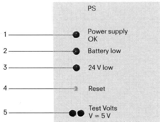
Fig. 19 Controls and displays on the power supply module
