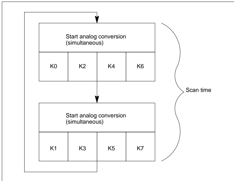
Figure 4-44 Hardware Filter 8 Channels Scan Time
