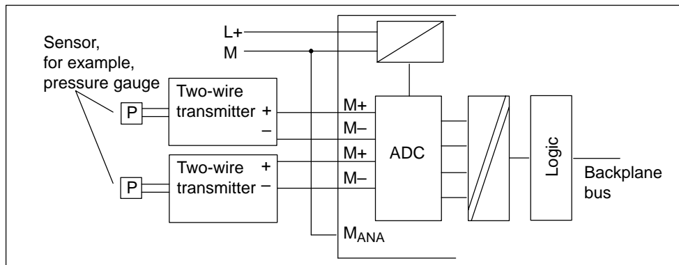
Figure 4-12 Connecting Two-Wire Transmitters to an Isolated AI
