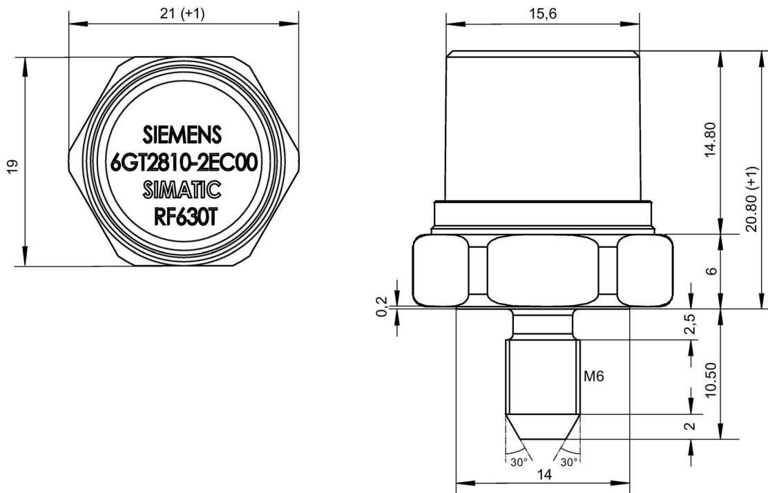
Figure 7-29 SIMATIC RF630T
