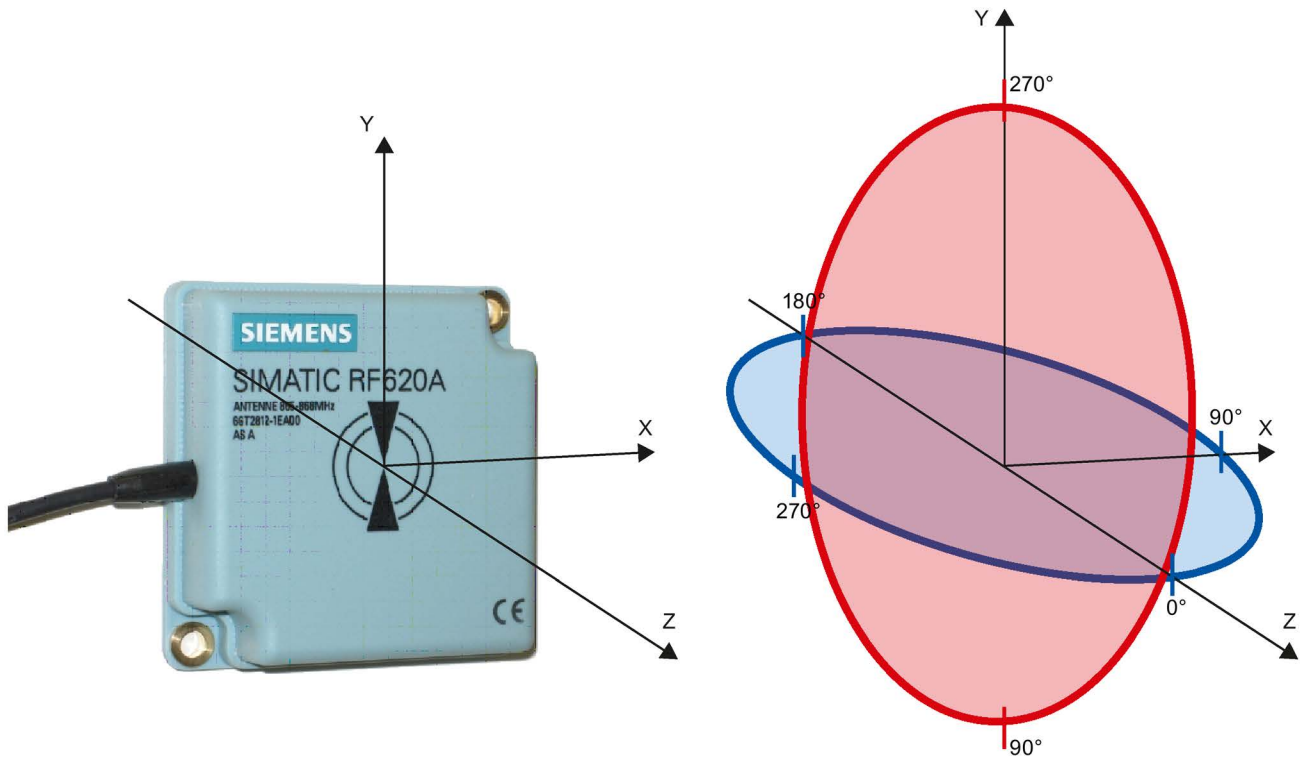
Figure 6-5 Reference system
