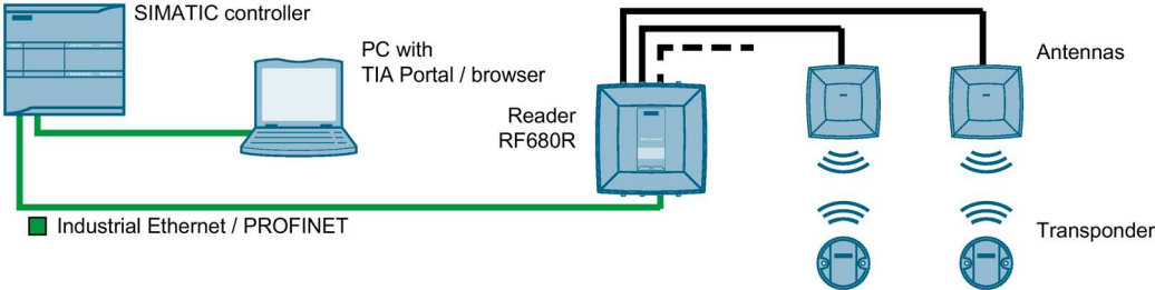
Figure 8-2 Configuration graphic with SIMATIC RF680R and PROFINET connection
