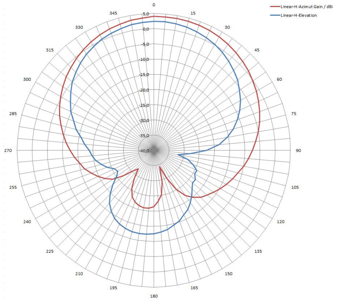
Figure 5-30 Elevation section
