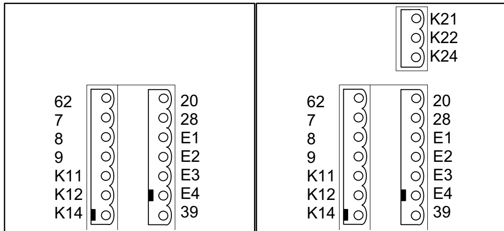
FIG 4-23 Layout of the control terminals
