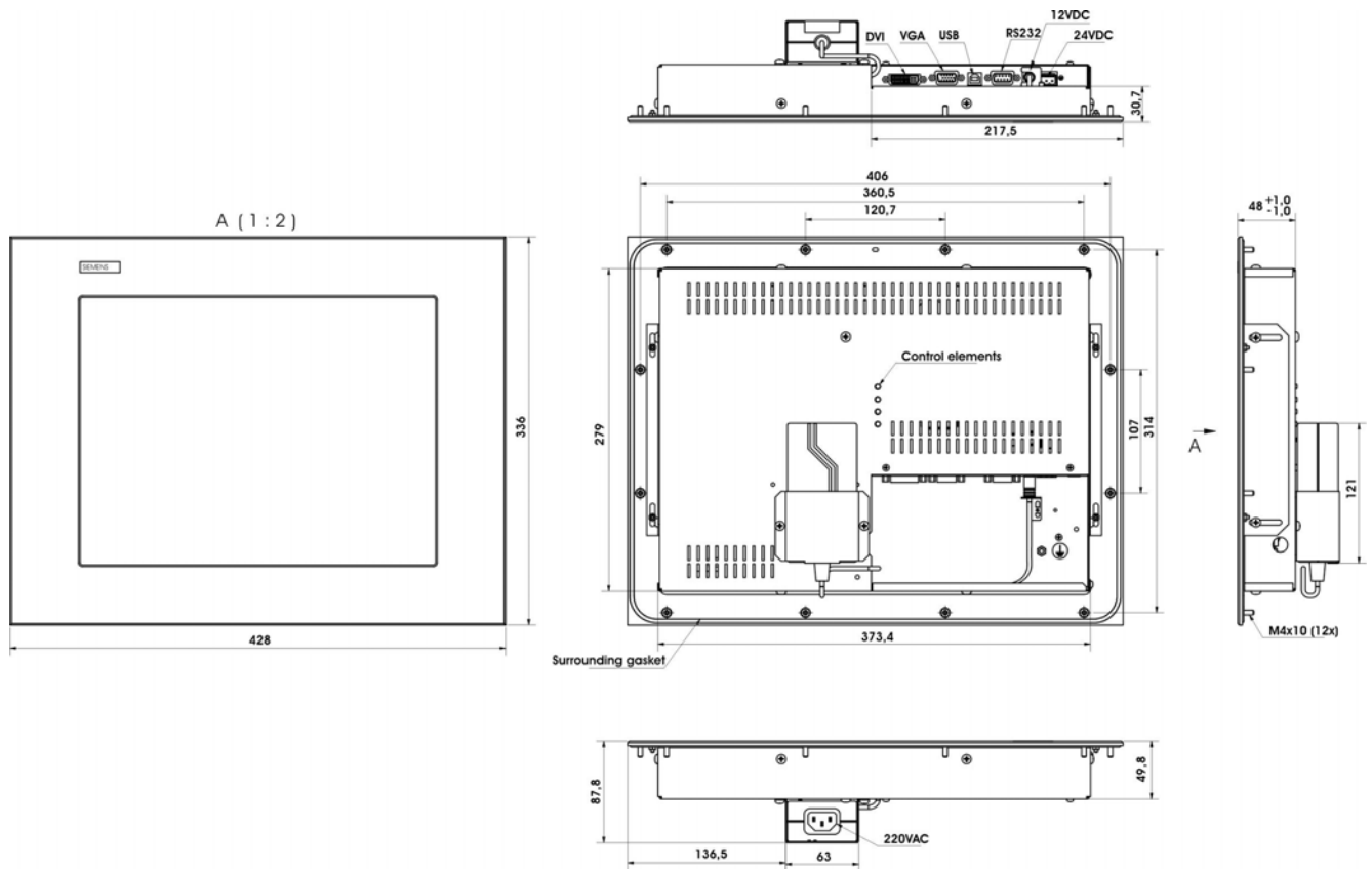
Fig. 1: Dimensions of the SCD 1597-E/ET
