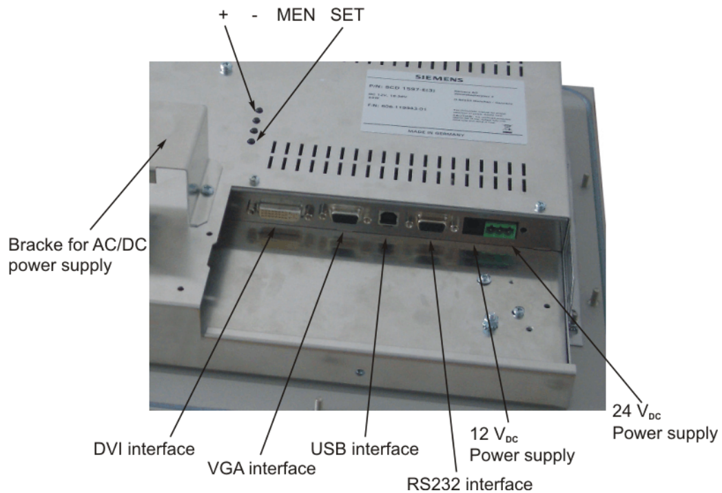
Fig. 3: Location of the operation and alignment controls
