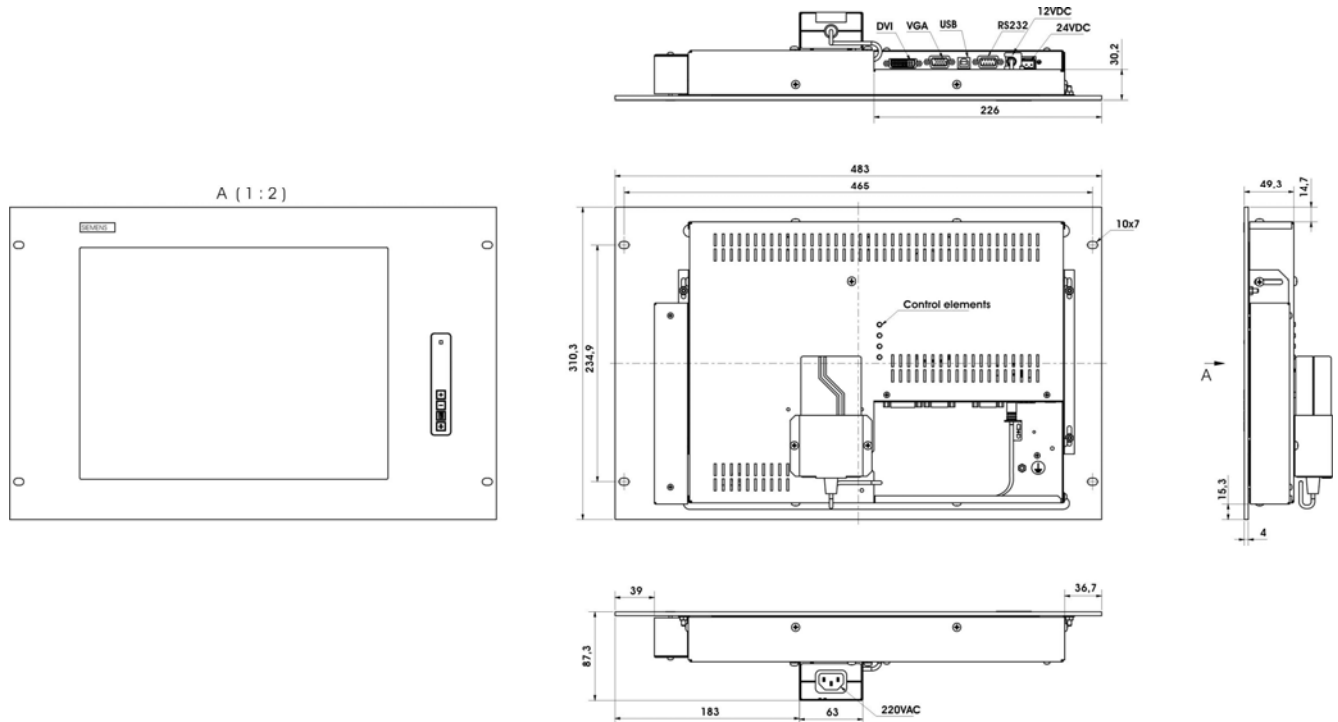
Fig. 2: Dimensions of the SCD 1597-R/RT
