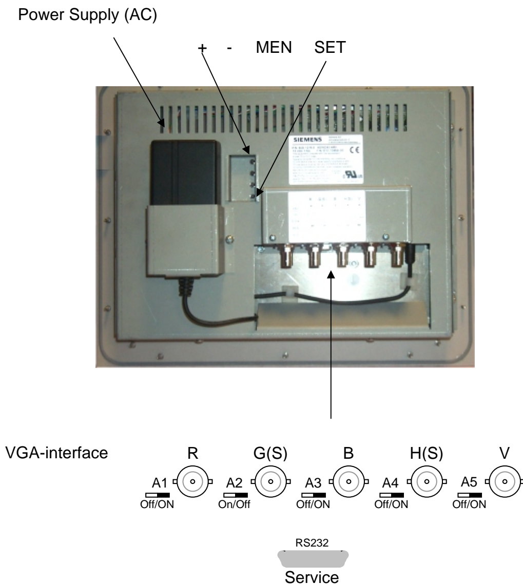
Fig. 2: Location of the interface and alignment control of the SCD 1215-E
