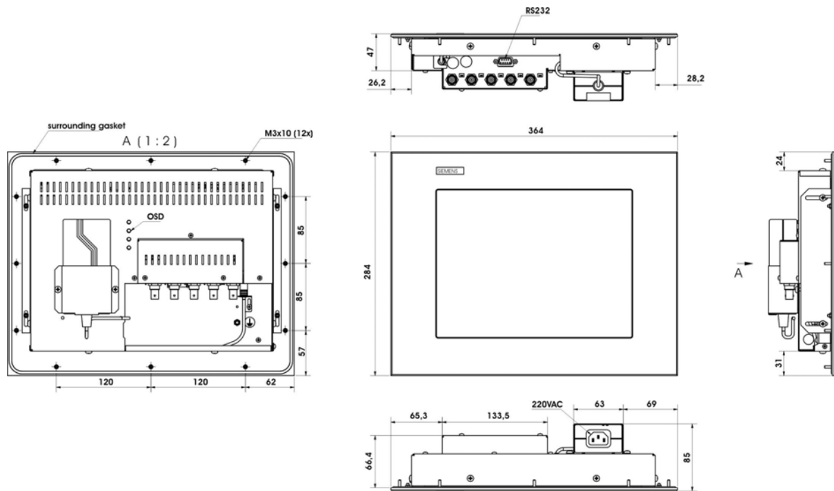
Fig. 1: Dimension of SCD 1215-E
