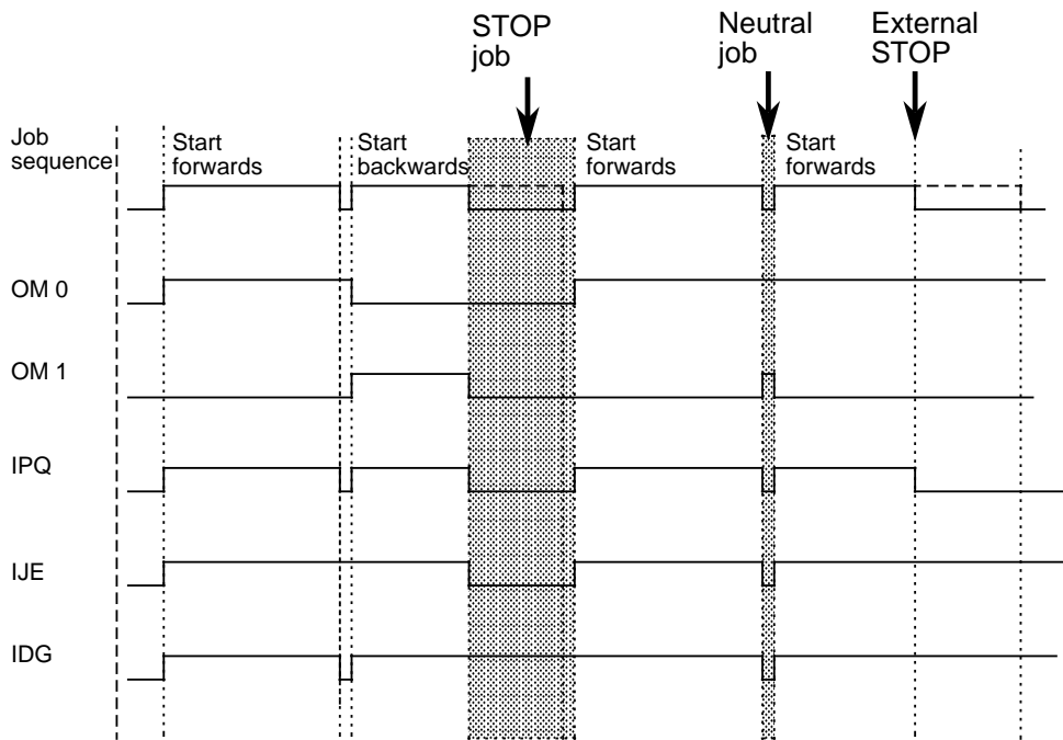
Figure 4-2. Operating Modes Diagram
