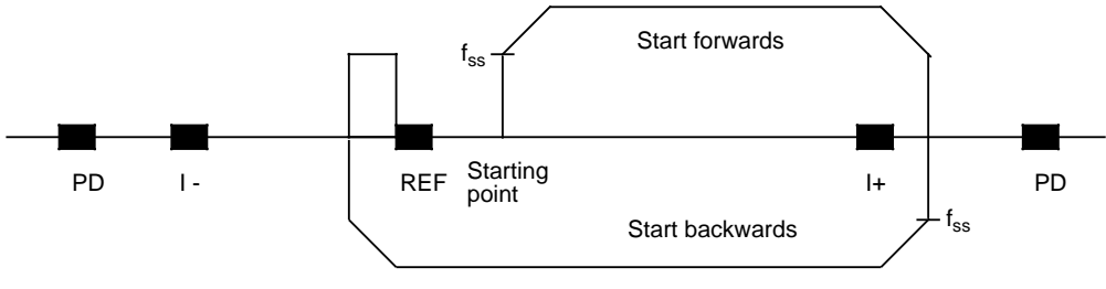
Figure 5-4. Reference Point Calculation with the REF Switch
