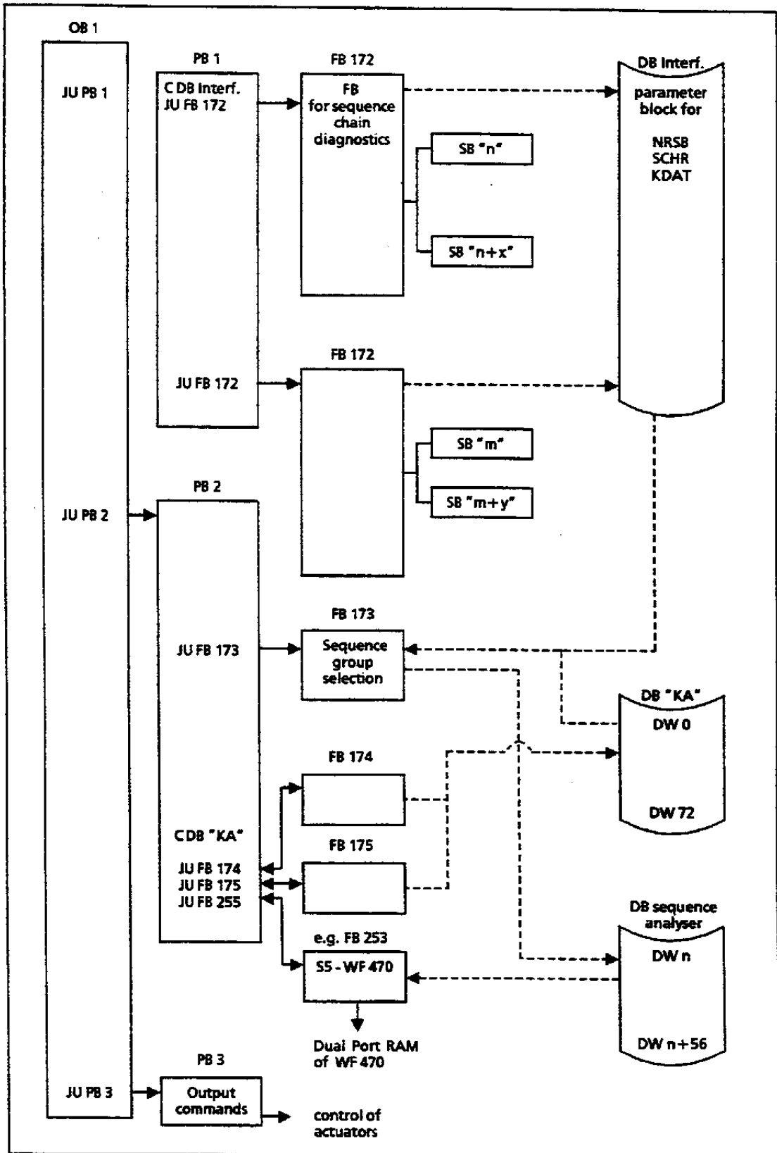
Fig. 3.4 Program structure
