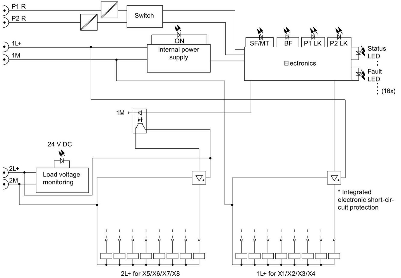
Figure 9-8 Block diagram of the 16 DO DC 24V/1,3A 8xM12 I/O device
