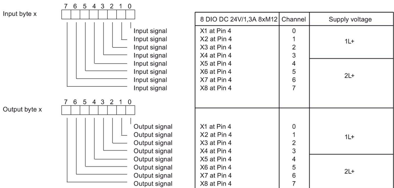
Figure E-8 Address space of 8 DIO DC 24V/1,3A 8xM12 I/O device
