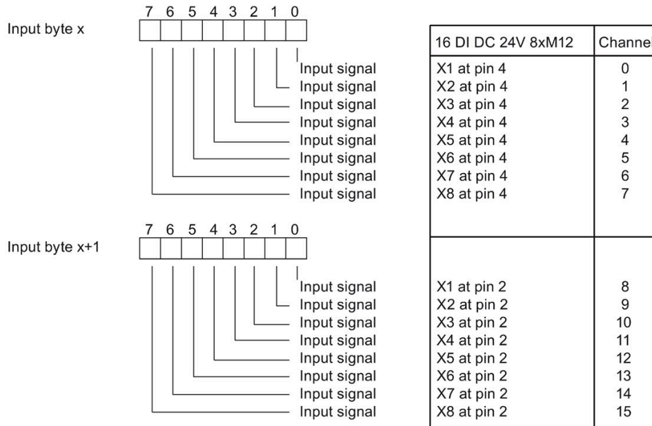
Figure E-3 Address space of 16 DI DC 24V 8xM12 I/O device
