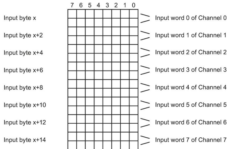
Figure E-10 Address space of 8 AI RTD/TC 8×M12 I/O device
