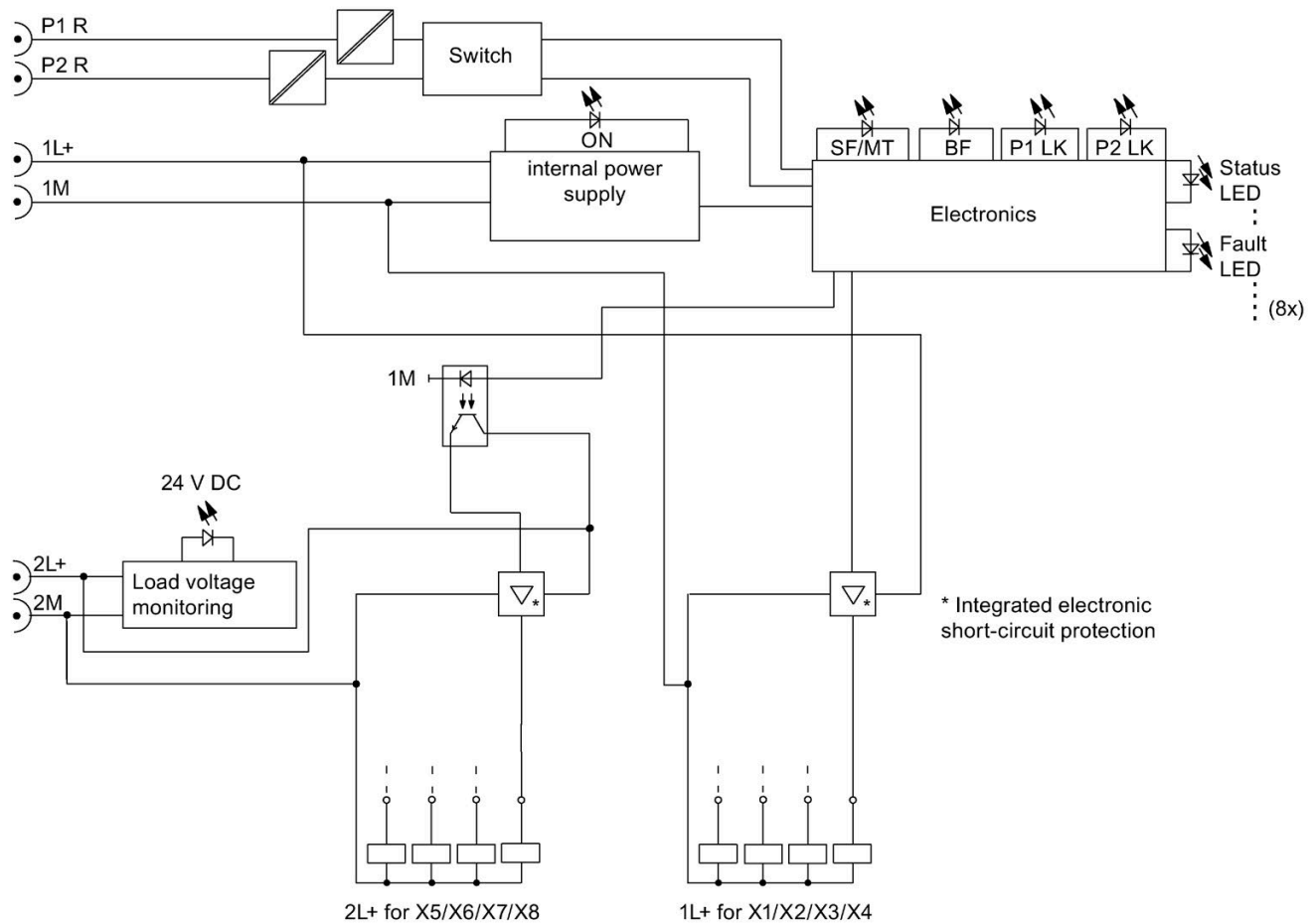
Figure 9-7 Block diagram of the 8 DO DC 24V/2,0A 8xM12 I/O device
