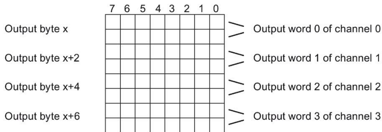
Figure E-11 Address space of 4 AO UI 4xM12 I/O device
