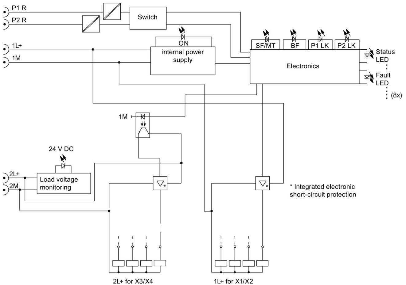
Figure 9-4 Block diagram of the 8 DO DC 24V/1,3A 4xM12 I/O device
