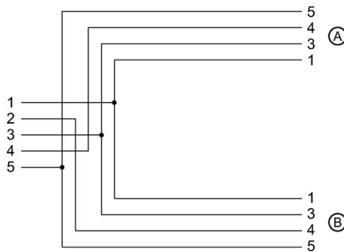
Figure 3-3 Y cable
