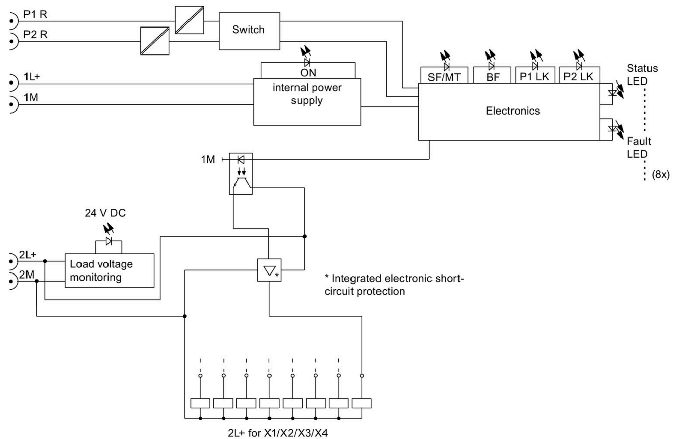
Figure 9-5 Block diagram of the 8 DO DC 24V/0,5 A 4xM12 I/O device
