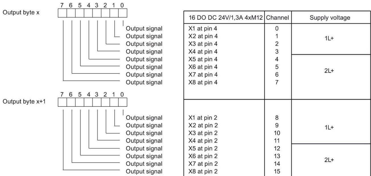
Figure E-7 Address space of 16 DO DC 24V/1,3A 8xM12 I/O device
