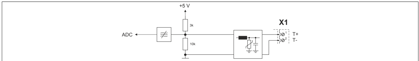
Figure 6: Temperature sensor
