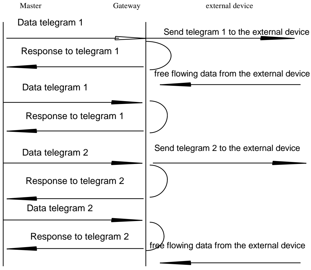
Figure 2: Data communication
