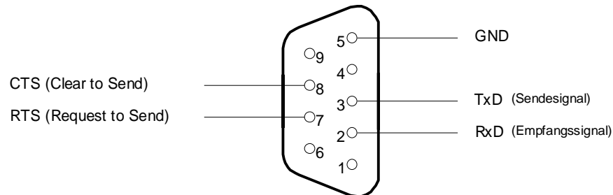
Figure 2: "RS 232C" communication interface
